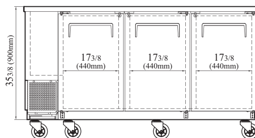
TBB-24-72SB-N6 FRONT VIEW
